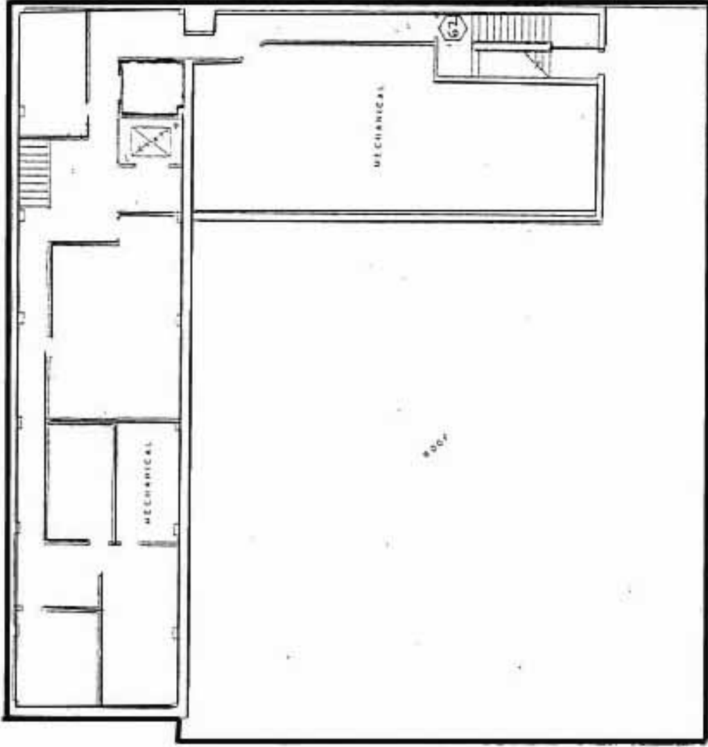
900 MONROE STREET PROFESSIONAL BUILDING FIFTH FLOOR PLAN
