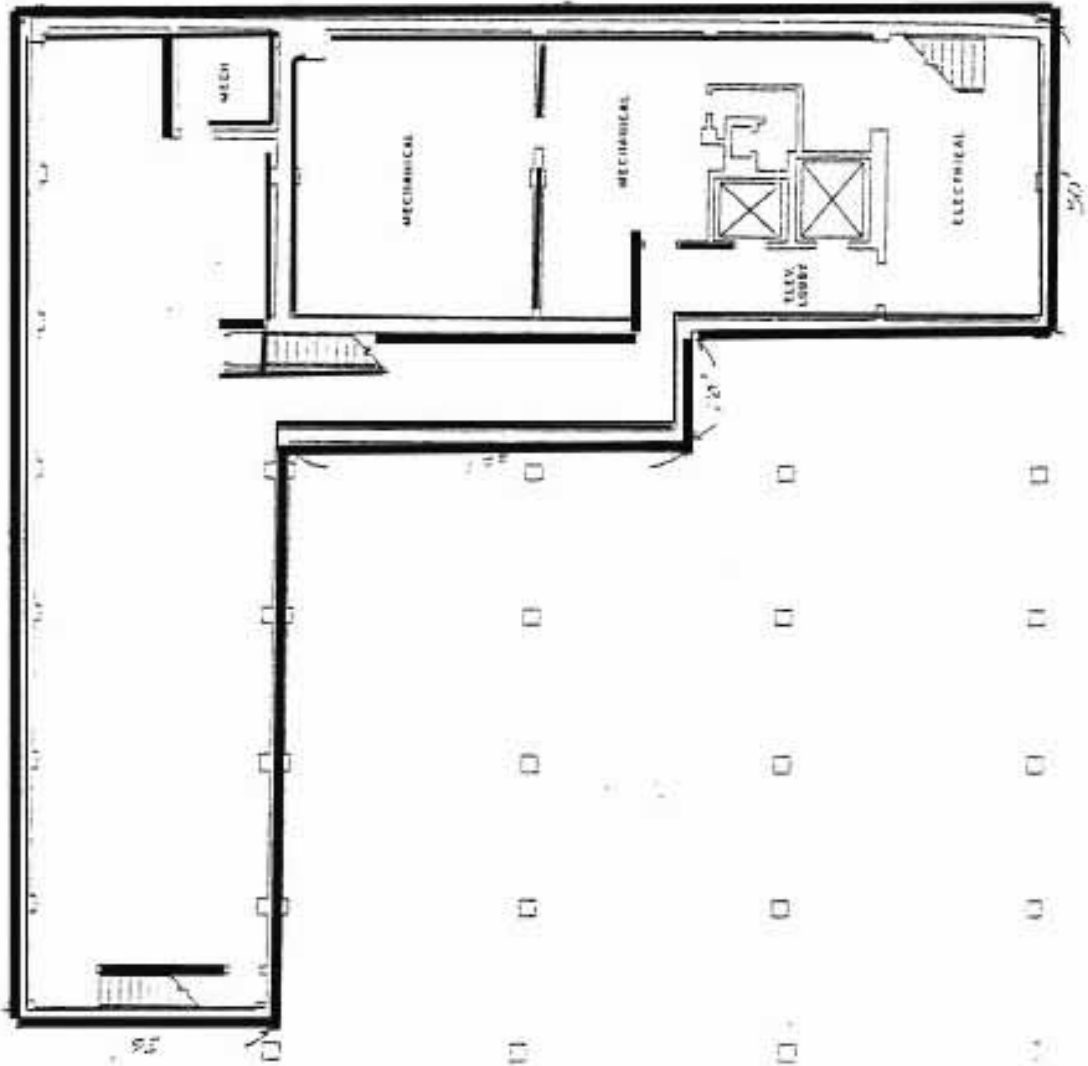
Basement Plan 900 Monroe Street Professional Building
